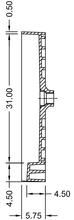
SECTION B-B
